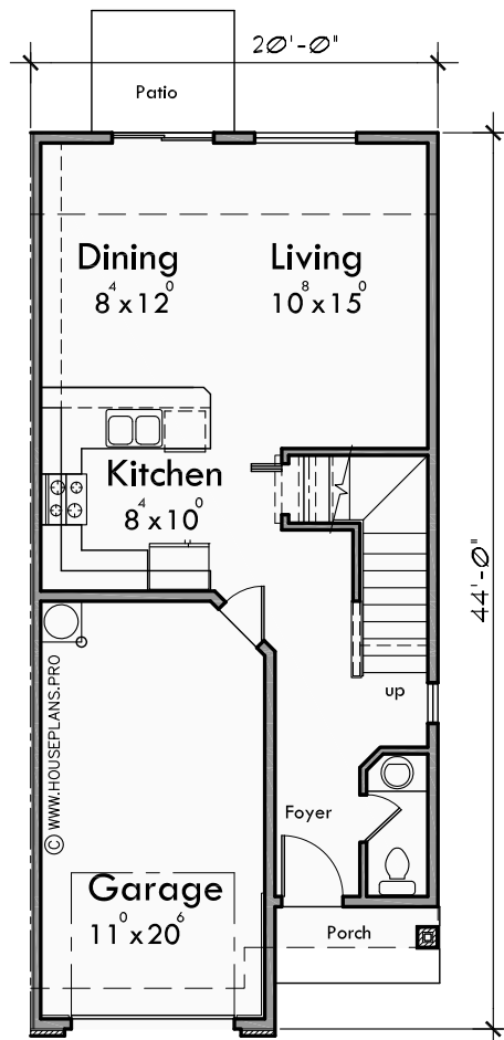
Main Floor
