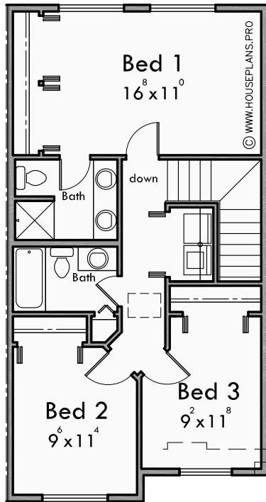
Upper Floor
