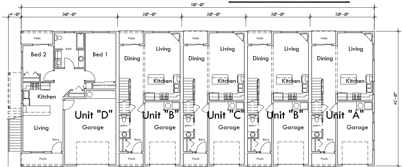
Main Floor 5 Unit Layout
