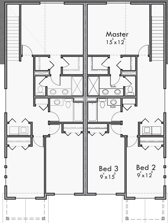
UPPER FLOOR
