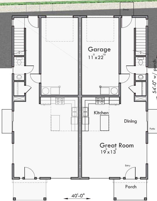
MAIN FLOOR
