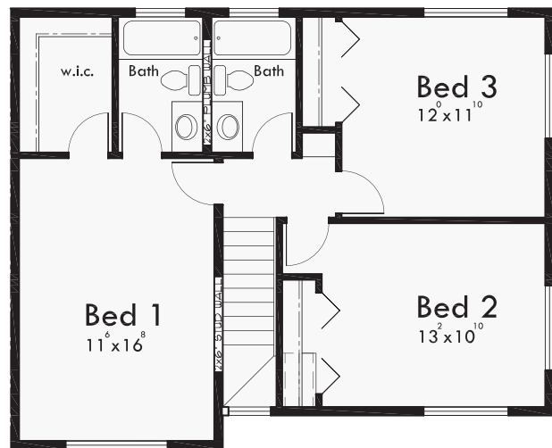
UPPER FLOOR
