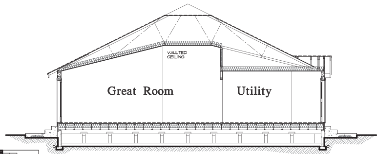
BUILDING SECTION
