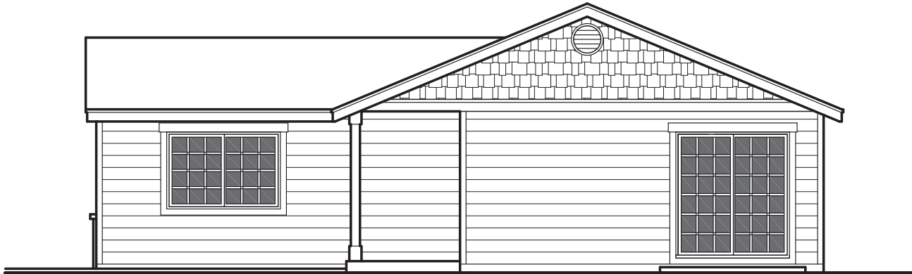
SIDE ELEVATION
