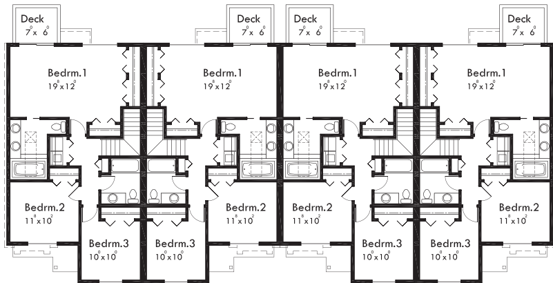
UPPER FLOOR
