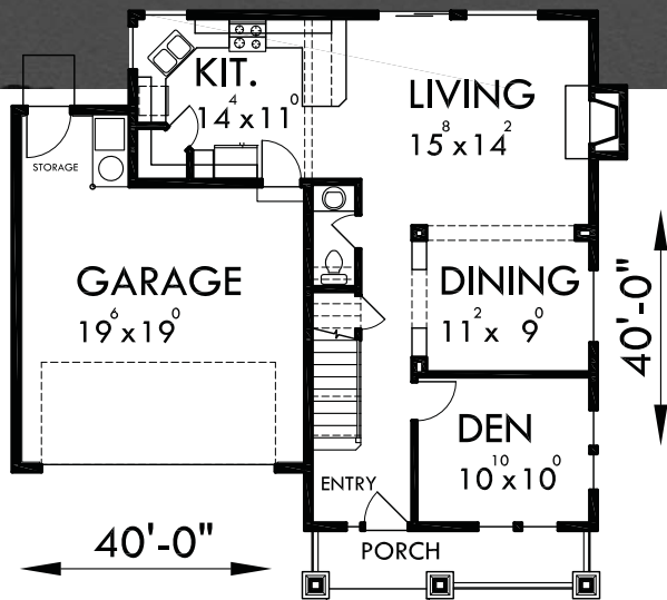
MAIN FLR.
