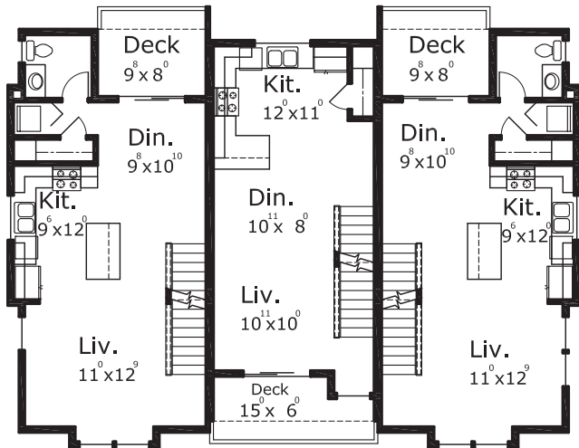
2ND FLOOR
