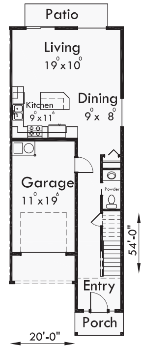
MAIN FLOOR
