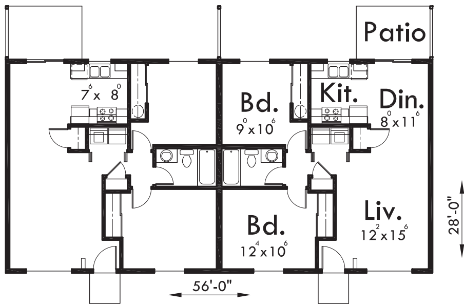
PLAN #D-024 EACH UNIT 784 SQ. FT.
