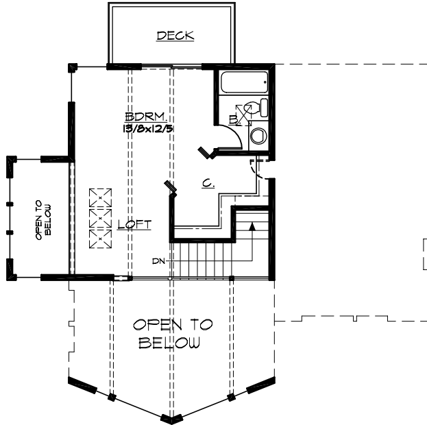
UPPER FLOOR
